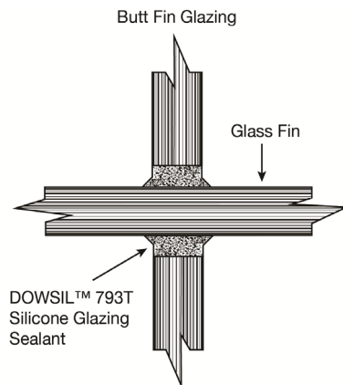
Figure 1: Sealing Glass with DOWSIL™ 793T Silicone Glazing Sealant.
